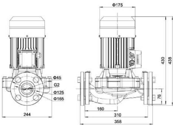
Three-phase
