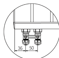
Compact Ventil
